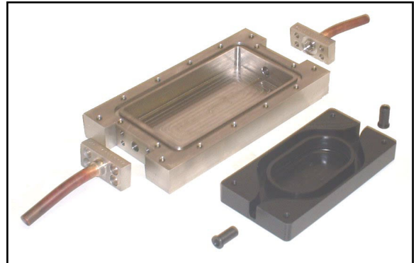
Stainless steel and nylon cable jointing box Dimensions 230mm x 125mm x 30mm
