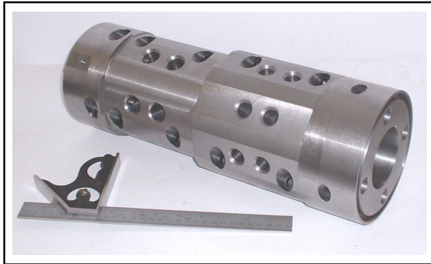
A mild steel multi-position indenting tool
